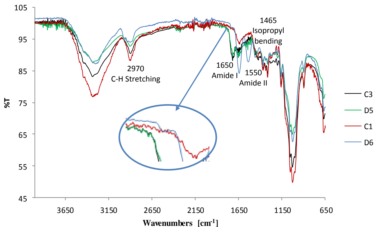
Figure 8: ATR-FTIR spectra of C3, D5, C1 and D6
