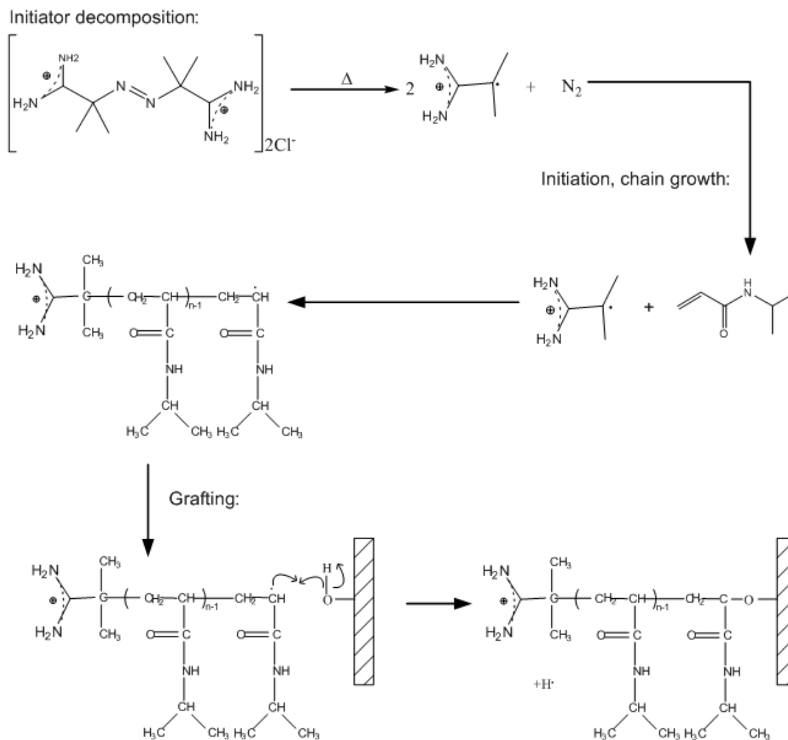
Figure 9: Reaction scheme showing the modification of cotton cellulose with microgels by grafting
