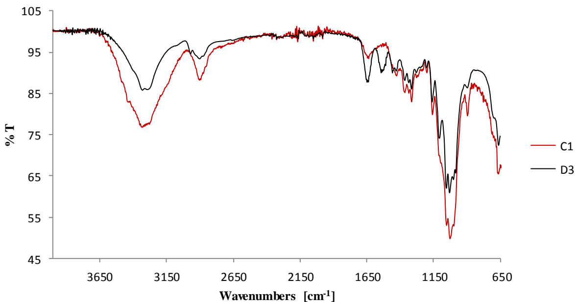
Figure 7: ATR-FTIR spectra of C1 and D3
