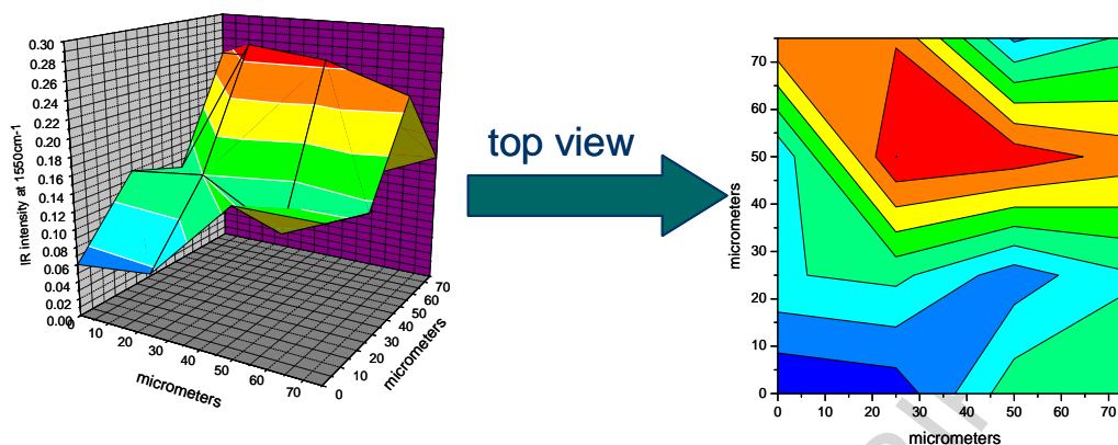
Figure 12: IR mapping of the sample D7
