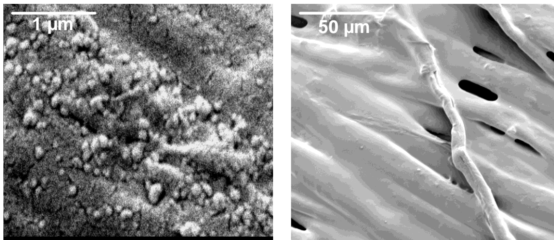
SEM images of cationic p(NIPAM) attached to blank cotton using polymer grafting.
