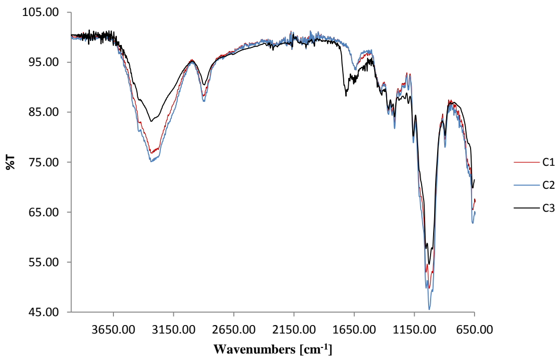
Figure 2: ATR-FTIR spectra of C1, C2 and C3
