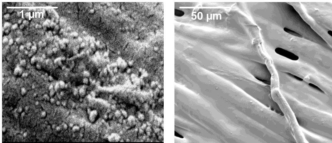
Figure 10: SEM images of D7
