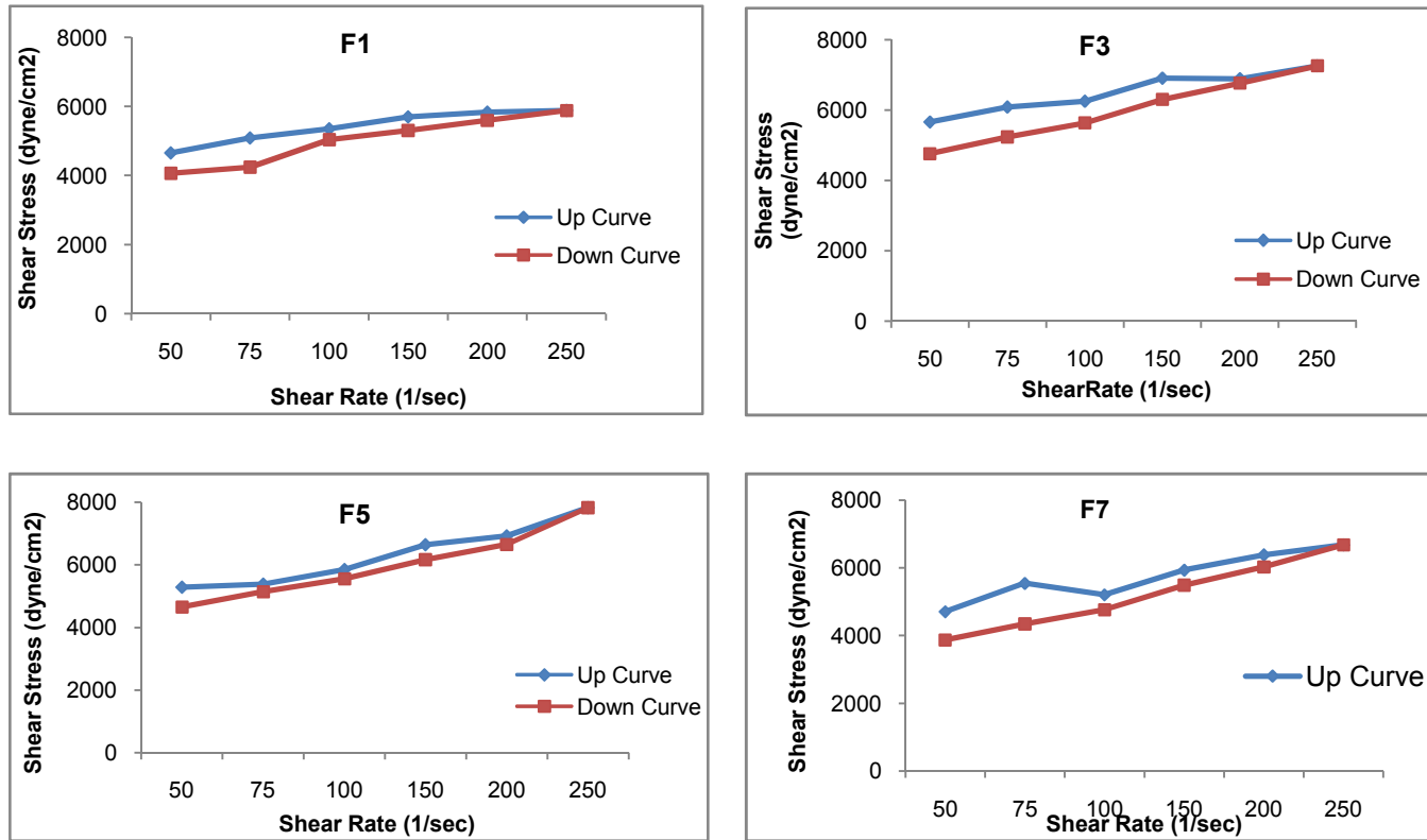
Fig. 3. Rheograms of Carbopol 934 Emulgel (F1, F3, F5 and F7)
