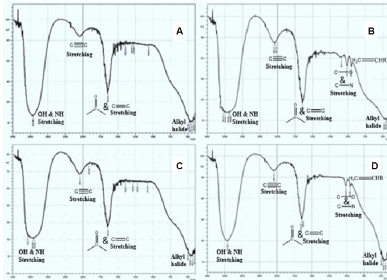
Figure 3 FTIR spectra after synthesis of nanoparticles of (A) Lampranthus coccineus aqueous extract, (B) Lampranthus coccineus hexane extract, (C) Malephora lutea aqueous extract, (D) Malephora lutea hexane extract.
