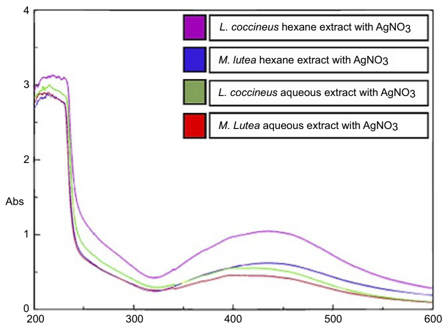
Figure 2 UV-Vis spectral analysis and color intensity of the biosynthesized SNPs of Lampranthus coccineus and Malephora lutea aqueous and hexane extract with AgNO 3 .
