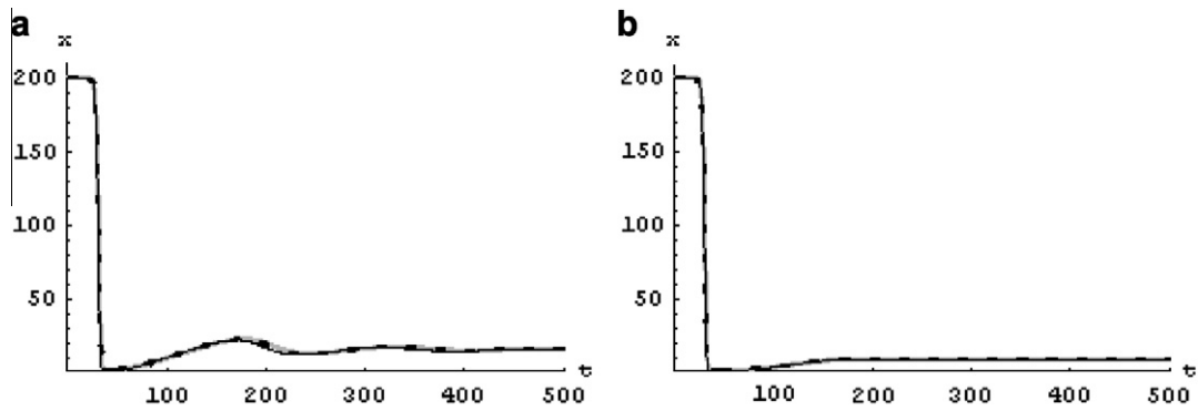
Fig. 1. The densities of the uninfected CD4^+ T-cells x(t) , when \varepsilon = 0.1 (a), and \varepsilon = 0.05 (b): gray solid line ( \alpha = 1 ), dotted line ( \alpha = 0.99 ), black solid line ( \alpha = 0.95 ).
