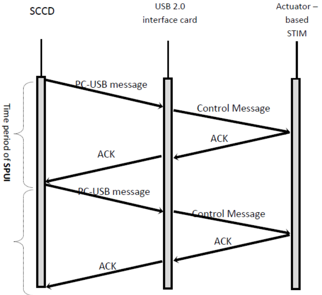
Fig.15 Communication scenario between SCCD and actuator-based STIM
