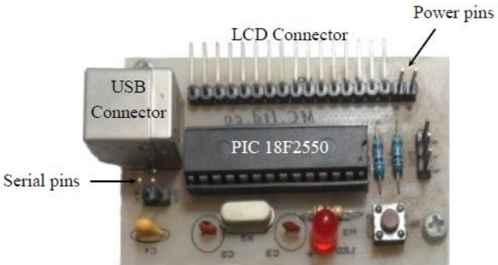
Fig.7 Practical circuit of USB 2.0 interface Card
