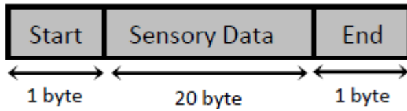
Fig.3 Format of Sensory Data Message (SDM)
