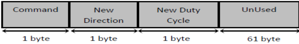
Fig.9 Format of PC-USB message
