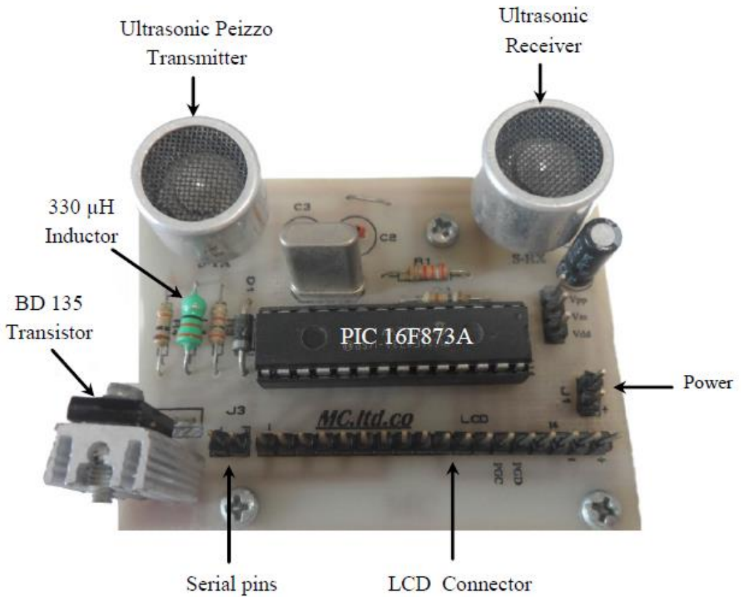
Fig.6 Practical circuit of MMD
