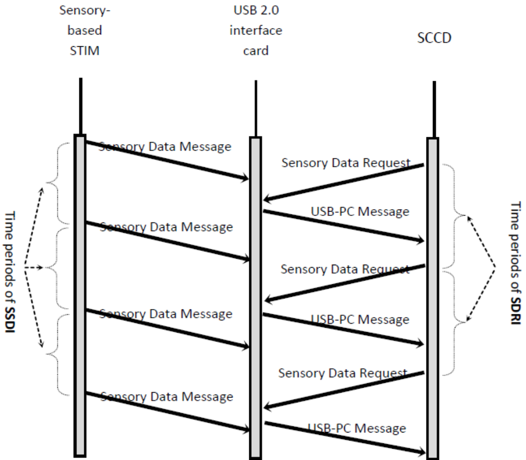
Fig.14 Communication scenario between SCCD and sensor-based STIM
