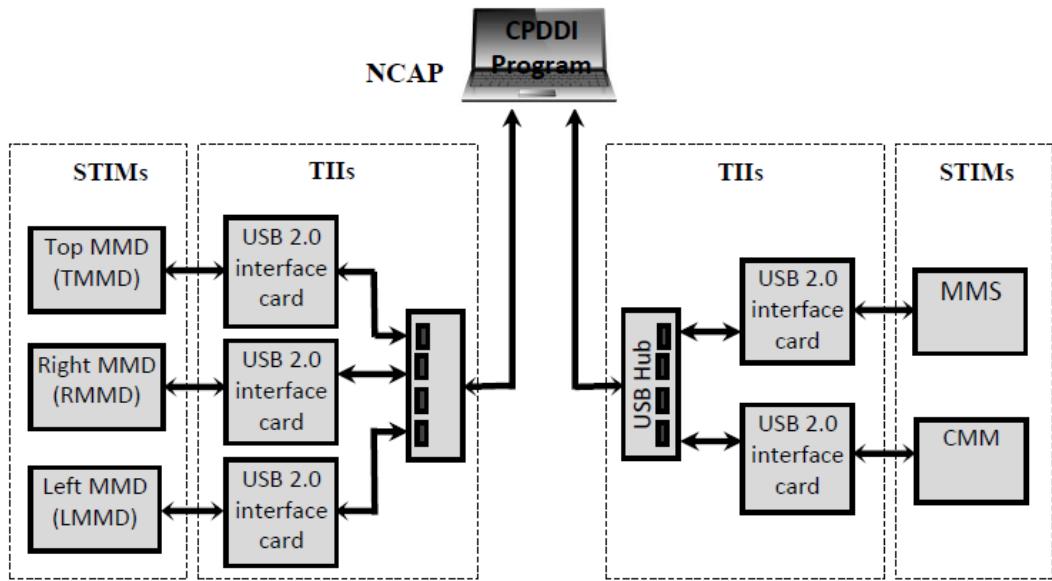
Fig.16 Practical test-bed for USANet system
