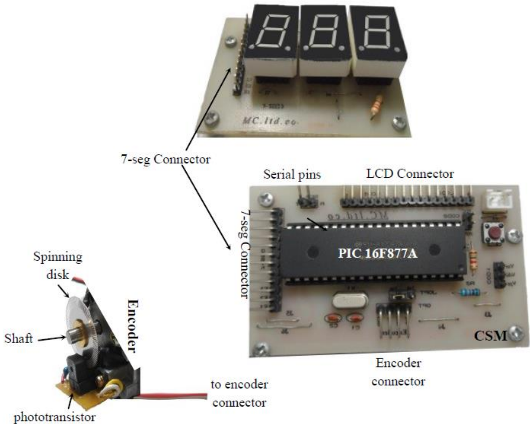
Fig.2 Practical three parts (sub-circuits) of MMS
