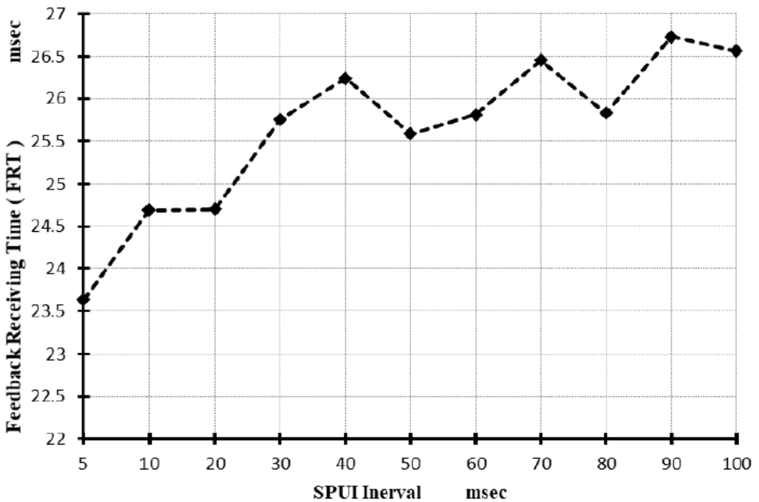
Fig.17 Practical results of Feedback Receiving Time (FRT) for USANet with 5 STIMs at different SPUI intervals
