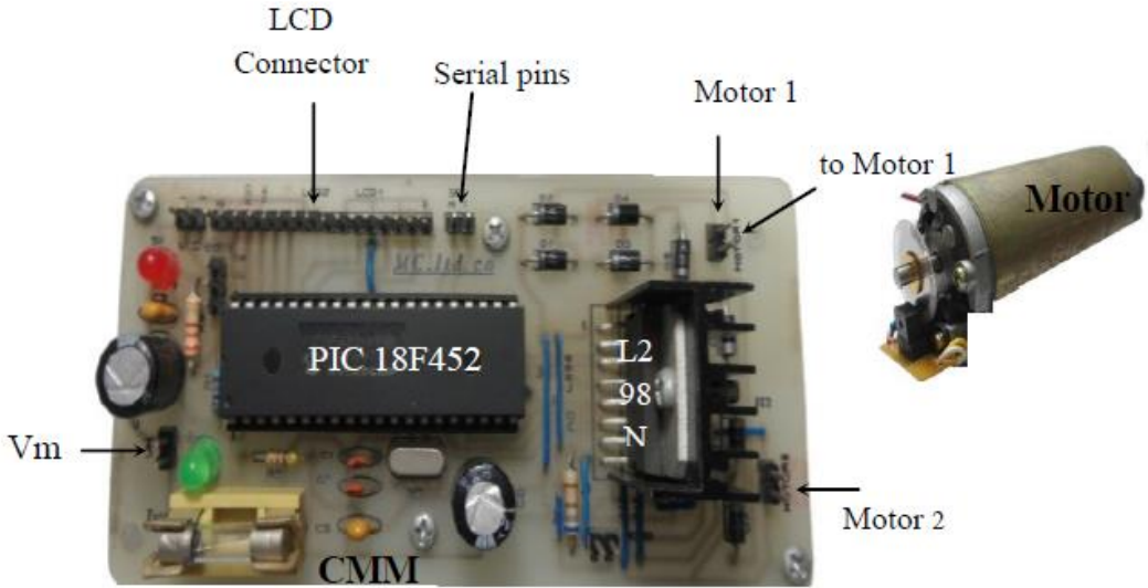
Fig.4 Practical circuit of CMM
