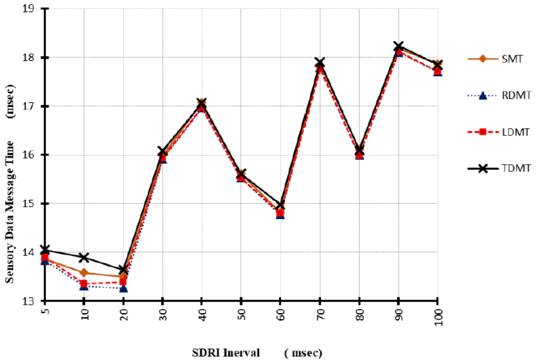
Fig.18 Practical results of SMT, RDMT, LDMT, and TDMT for USANet with 5 STIMs at different SDRI intervals
