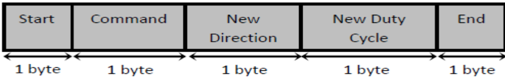
Fig.5 Format of Control Message
