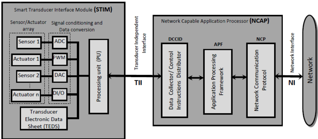
Fig.1 Key components of IEEE 1451 standard
