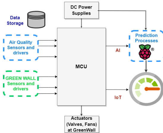
Fig.14 Proposed Schematic Control Scheme
