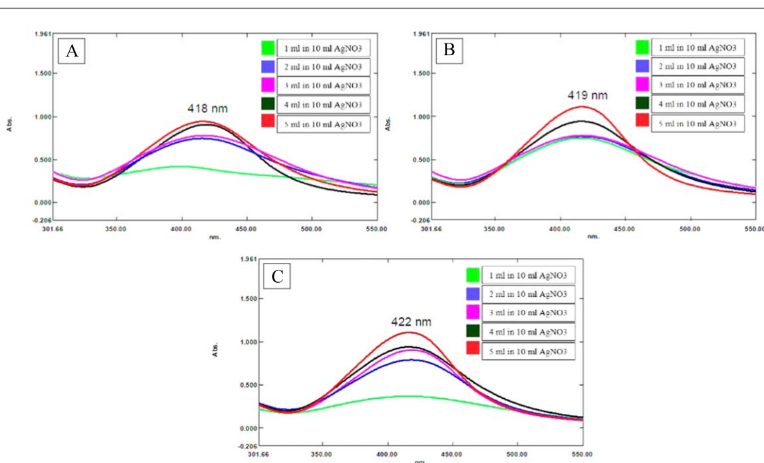
Figure 3. UV-visible spectroscopic analysis of the synthesized AgNPs at five different concentrations of P. crispum (A), S. maydis (B) and GA (C) solutions.
