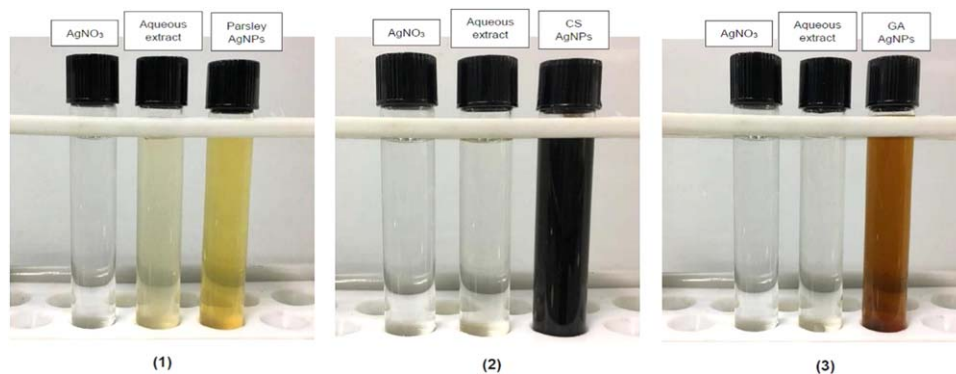
Figure 2. Early signs of AgNPs formation in (1) parsley, (2) CS and (3) GA aqueous extracts observed as the color of the solutions changed to yellowish-brown after 24 h of incubation with 1 mM \text{AgNO}_3 solution.
