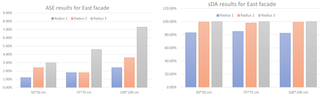
Fig. 8. Comparison of ASE and sDA for the East facade of the three simulation grids size. Source: the researchers
