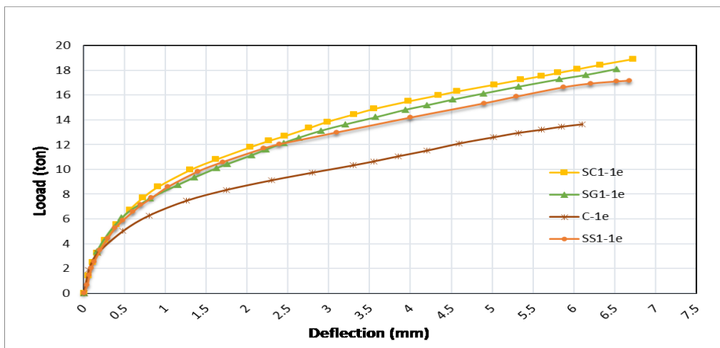
Fig. 10. Effect of using different strengthening materials (CFRP, GFRP& Steel links) in case of specimens strengthened by one row and loaded under eccentricity value (1e).
