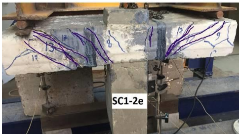
Fig. 34. Pattern of cracking for specimen (SC1-2e).
