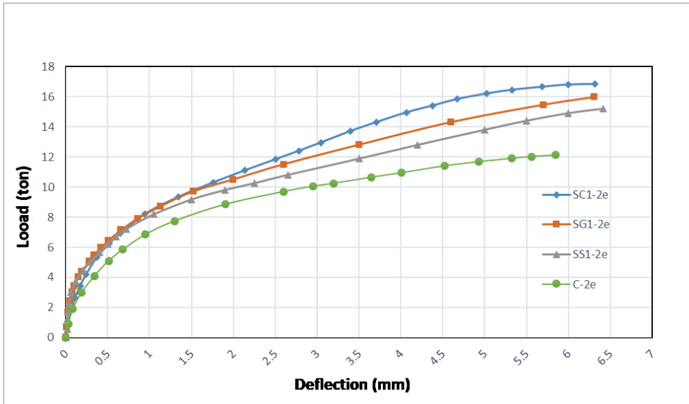
Fig. 11. Effect of using different strengthening materials (CFRP, GFRP& Steel links) in case of specimens strengthened by one row and loaded under eccentricity value (2e).
