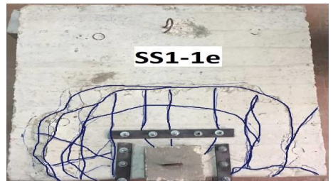
Fig. 41. Pattern of cracking for specimen (SS1-1e).
