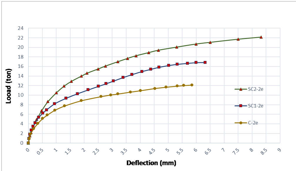
Fig. 15. Effect of rows number of (CFRP) strengthening stirrups with eccentricity value (2e).
