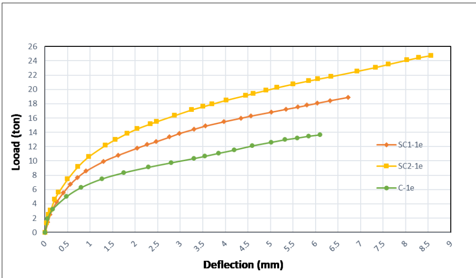
Fig. 14. Effect of rows number of (CFRP) strengthening stirrups with eccentricity value (1e).
