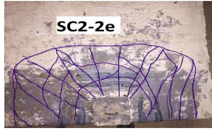
Fig. 36. Pattern of cracking for specimen (SC2-2e).
