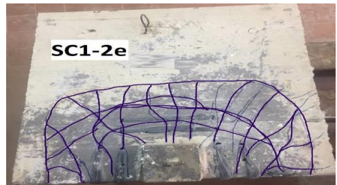
Fig. 34. Pattern of cracking for specimen (SC1-2e).
