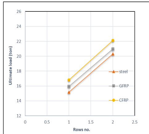
Fig. 27. Number of rows effect with 2e.
