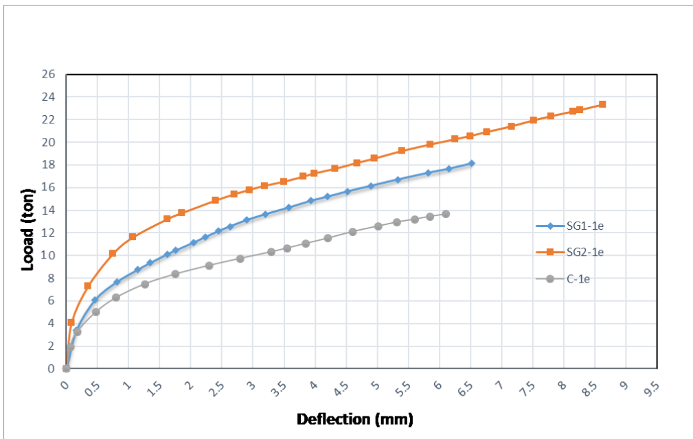
Fig. 16. Effect of rows number of (GFRP) strengthening stirrups with eccentricity value (1e).
