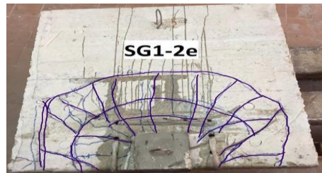
Fig. 38. Pattern of cracking for specimen (SG1-2e).
