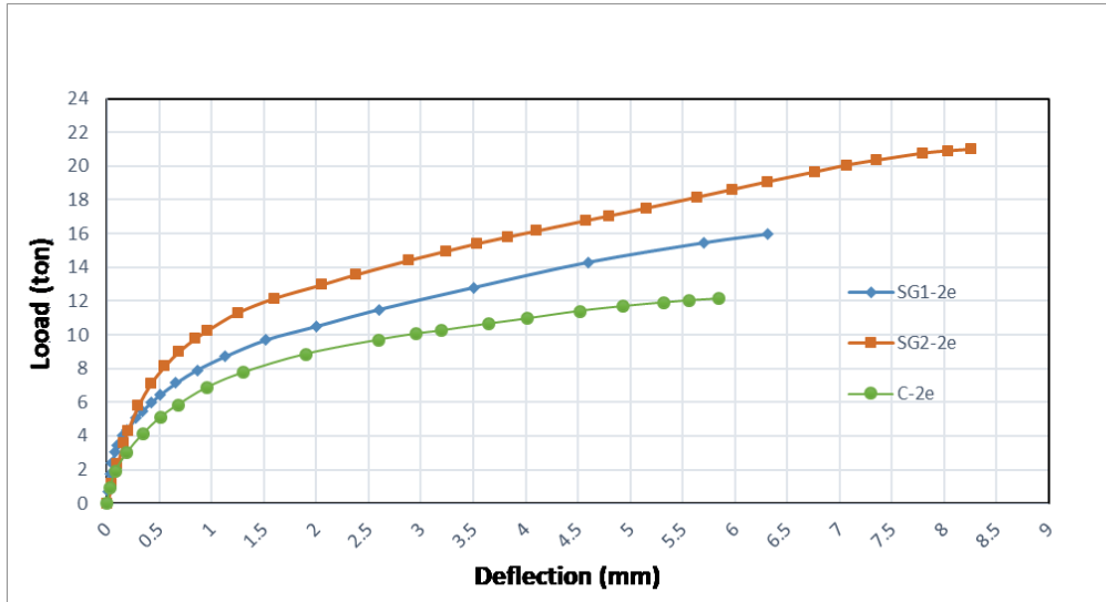
Fig. 17. Effect of rows number of (GFRP) strengthening stirrups with eccentricity value (2e).
