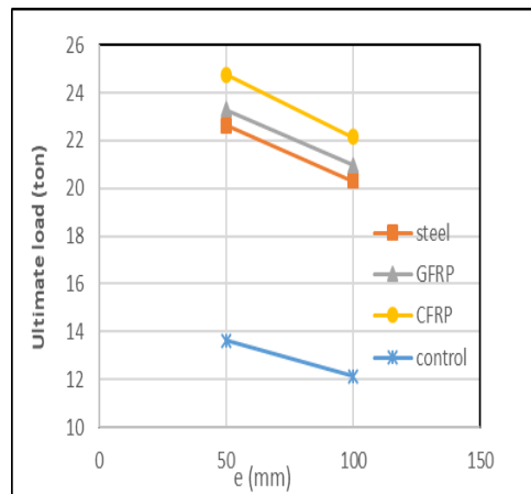
Fig. 29. The (e) value effect with two rows.
