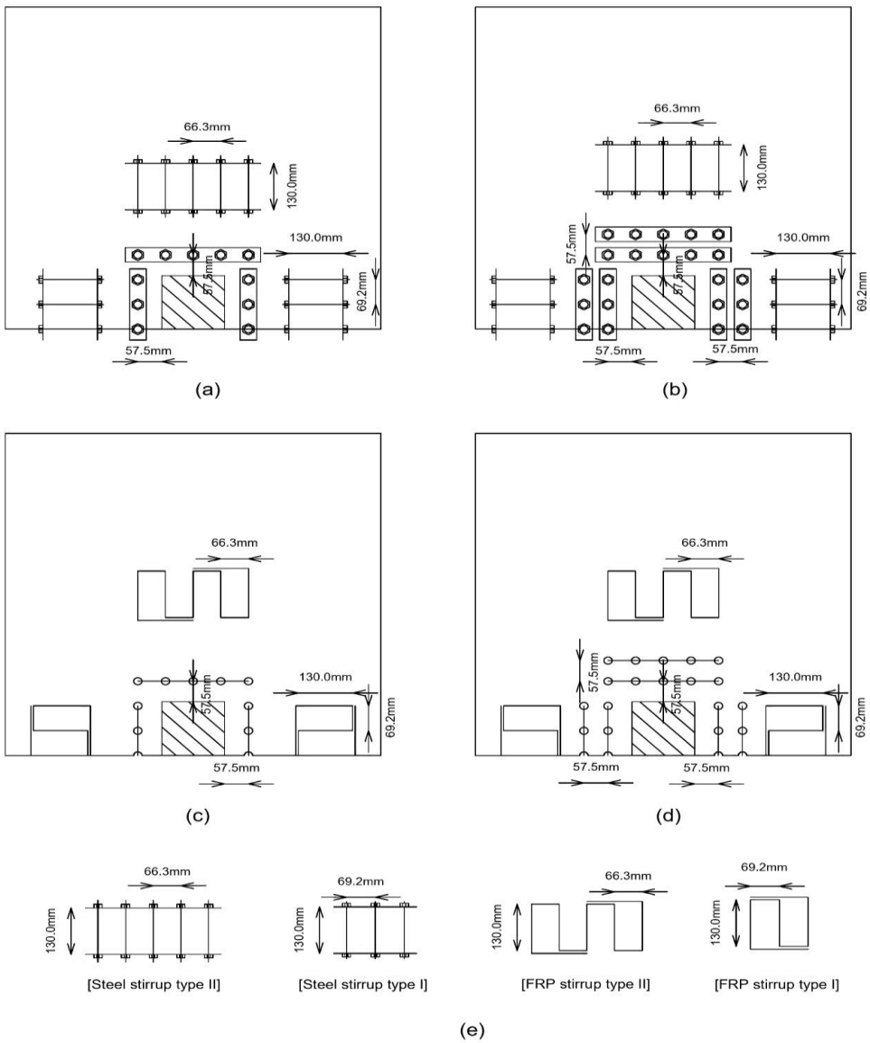
Fig. 5 Strengthening systems details; steel links using one row (a), two rows of steel (b), Using one row of FRP stirrups (c), Using two rows of FRP stirrups (d) stirrups types details (e).
