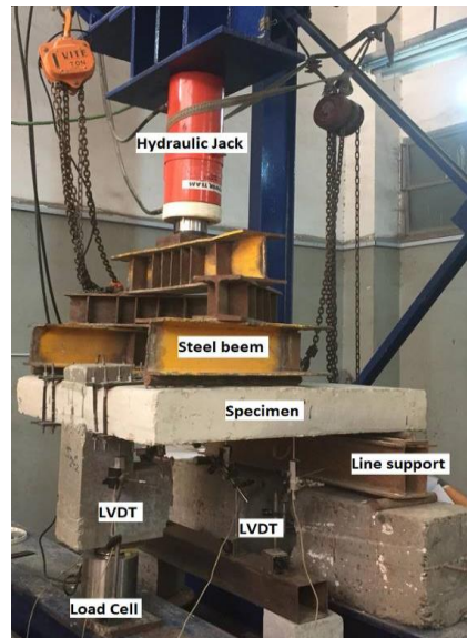
Fig. 9. Test set up.
