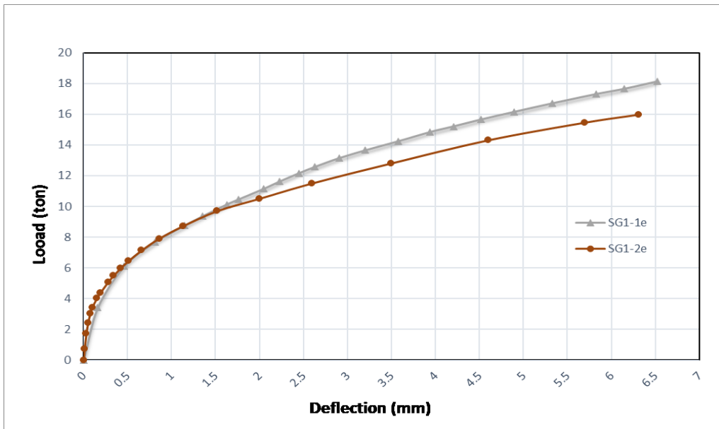
Fig. 22. Effect of load eccentricity value (e) variation with one row of (GFRP) strengthening stirrups.
