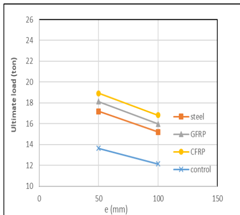
Fig. 28. The (e) value effect with one row.
