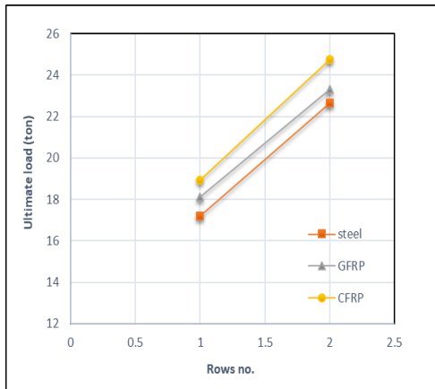
Fig. 26. Number of rows effect with 1e.
