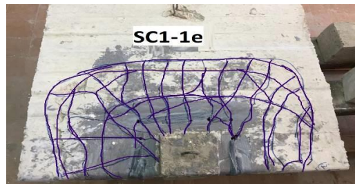
Fig. 33. Pattern of cracking for specimen (SC1-1e).
