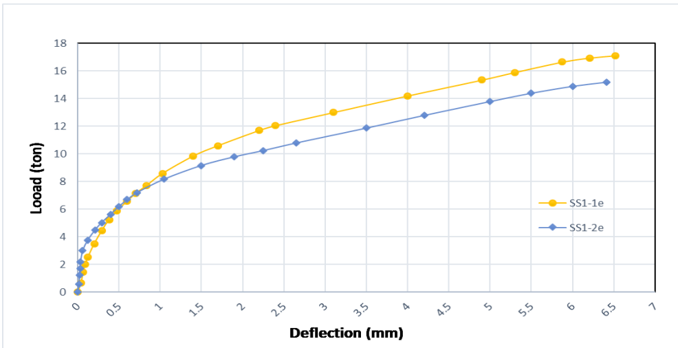
Fig. 24. Effect of load eccentricity value ( e ) variation with one row of strengthening steel links.
