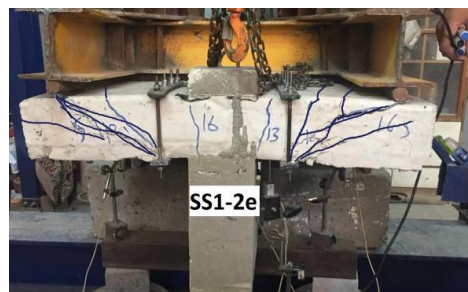
Fig. 43. Pattern of cracking for specimen (SS1-2e).
