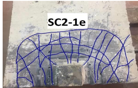
Fig. 35. Pattern of cracking for specimen (SC2-1e).
