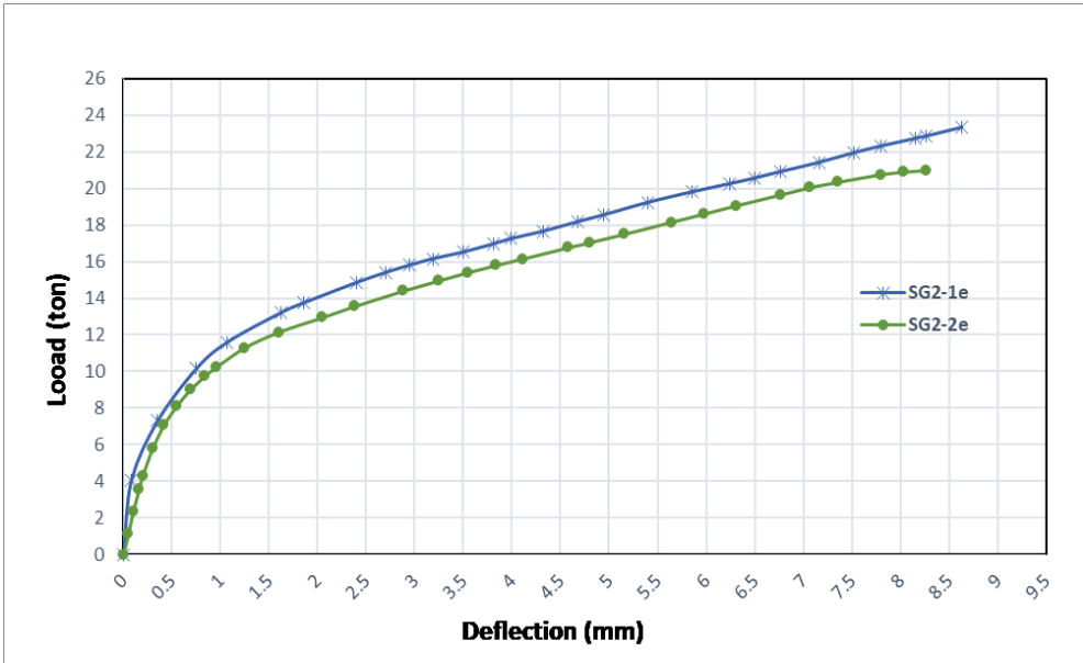
Fig. 23. Effect of load eccentricity value ( e ) variation with two rows of (GFRP) strengthening stirrups.
