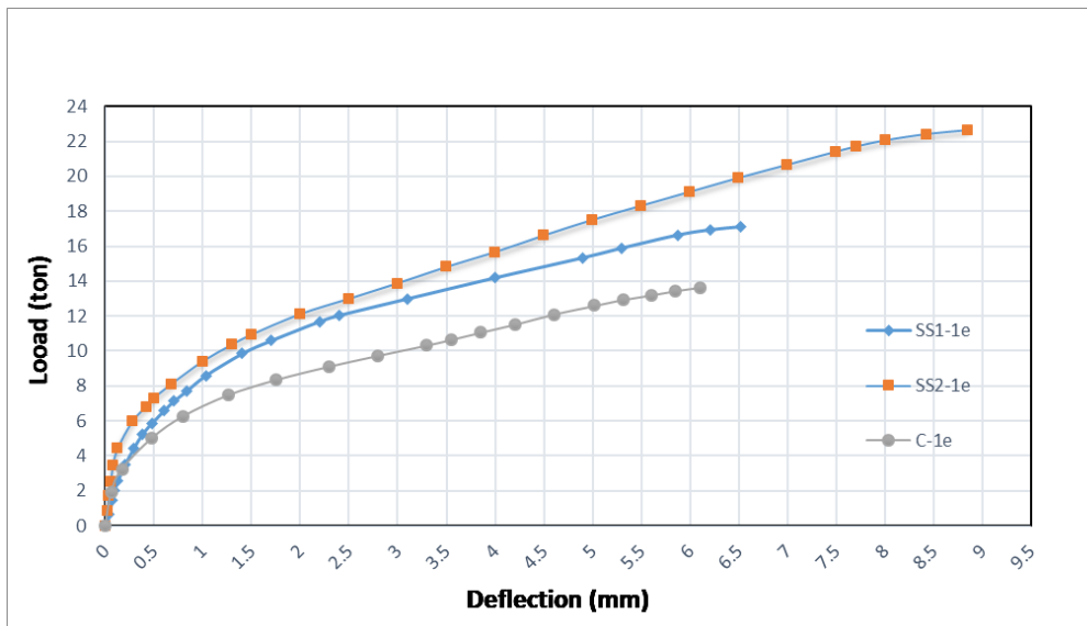
Fig. 18. Effect of rows number of strengthening steel links with eccentricity value (1e).
