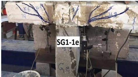
Fig.37. Pattern of cracking for specimen (SG1-1e).
