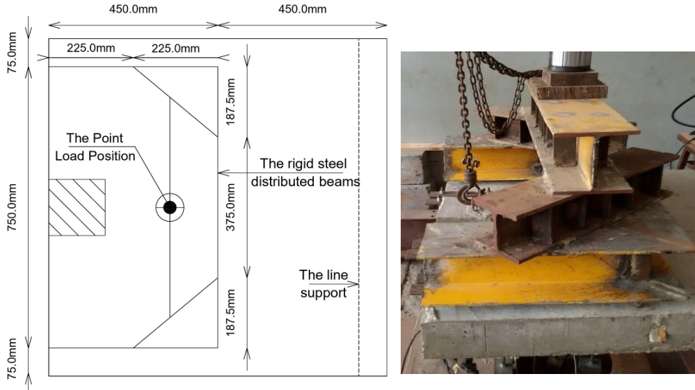
Fig. 7. The used distributed rigid steel beams.
