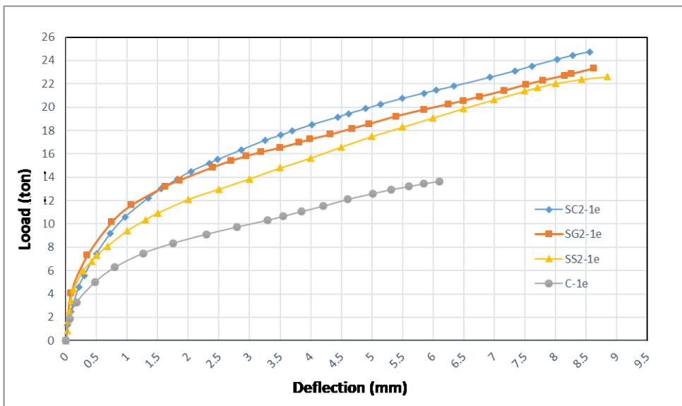
Fig. 12. Effect of using different strengthening materials (CFRP, GFRP& Steel links) in case of specimens strengthened by two rows and loaded under eccentricity value (1e).
