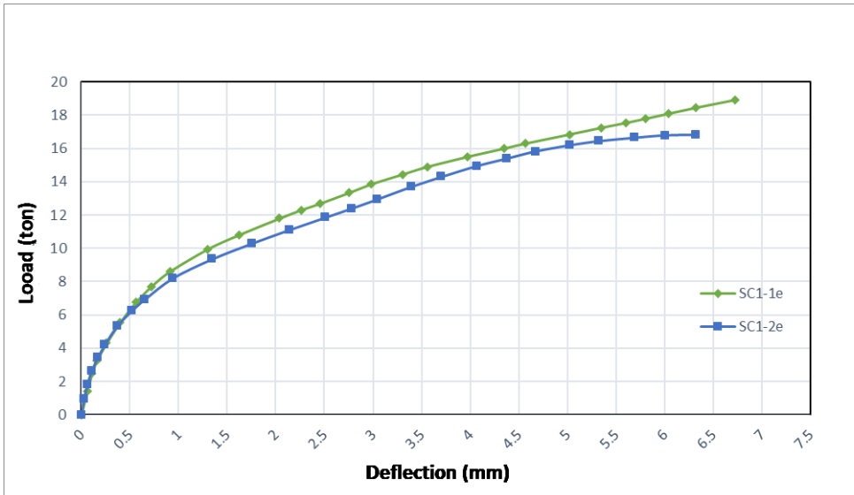
Fig. 20. Effect of load eccentricity value (e) variation with one row of (CFRP) strengthening stirrups.
