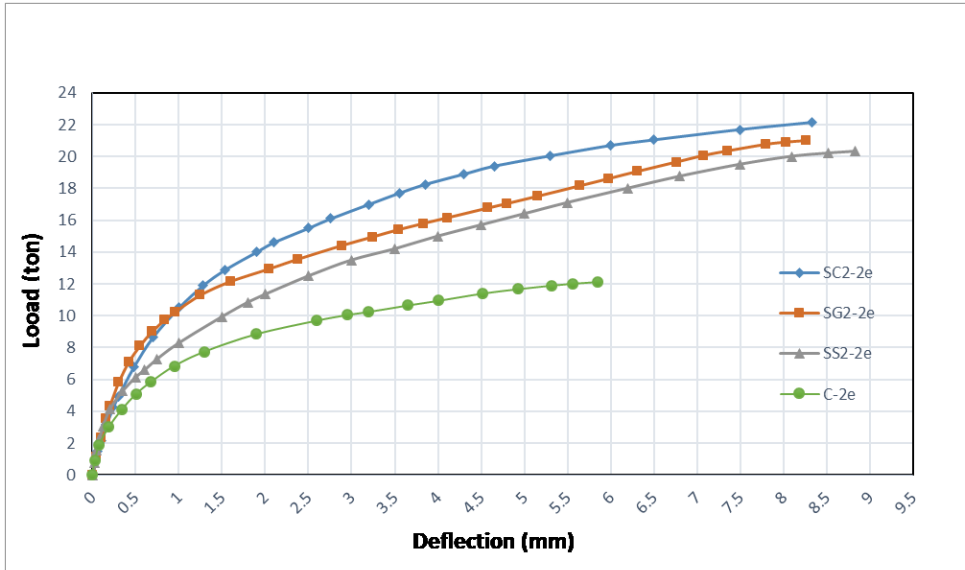
Fig. 13. Effect of using different strengthening materials (CFRP, GFRP& Steel links) in case of specimens strengthened by two rows and loaded under eccentricity value (2e).
