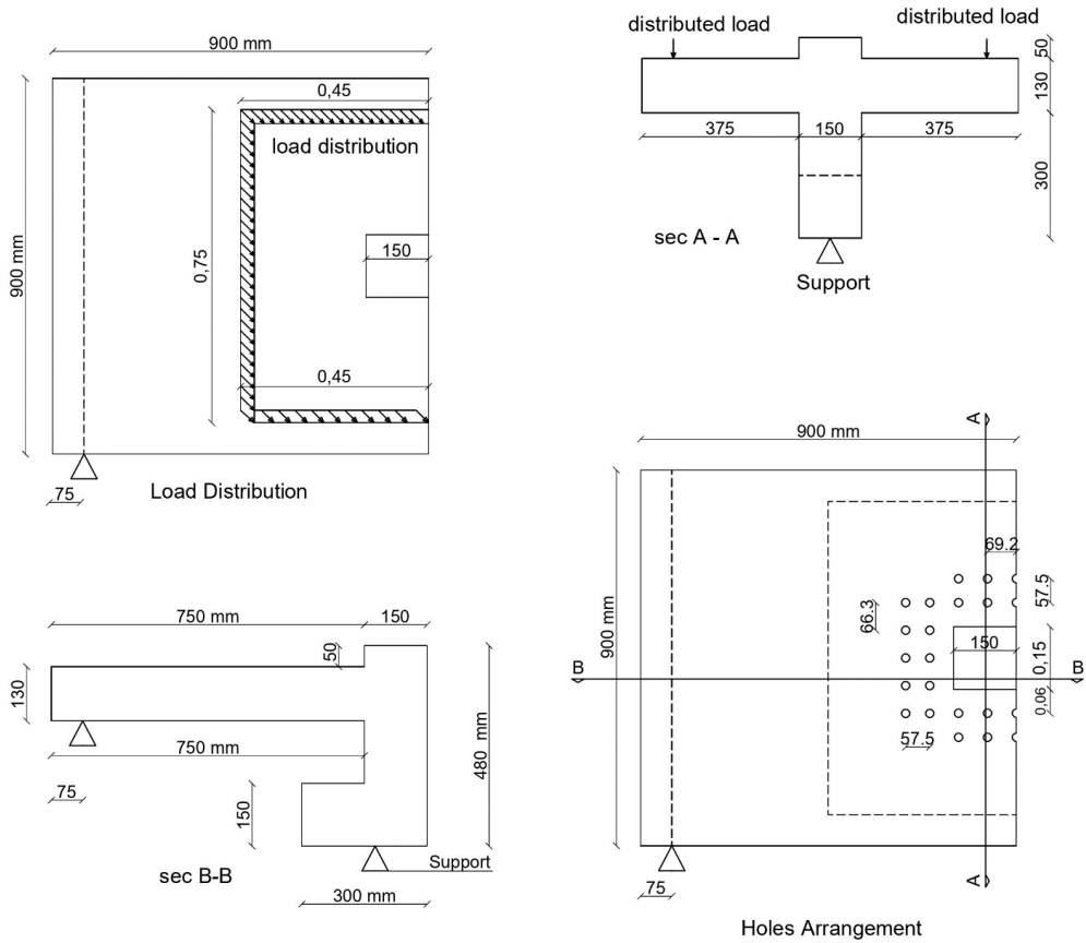
Fig. 1 The specimens' supports and dimensions.
