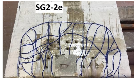
Fig. 40. Pattern of cracking for specimen (SG2-2e).
