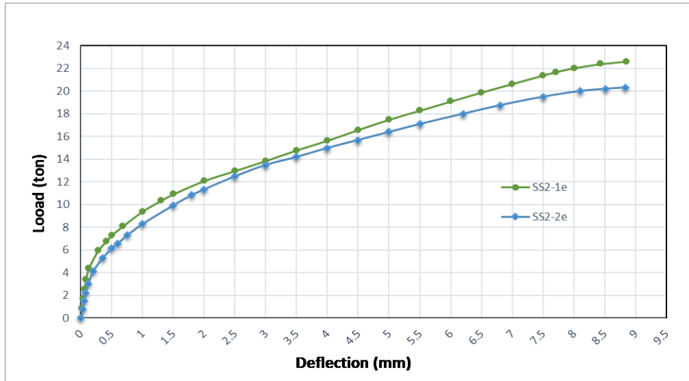
Fig. 25. Effect of load eccentricity value ( e ) variation with two rows of strengthening steel links.
