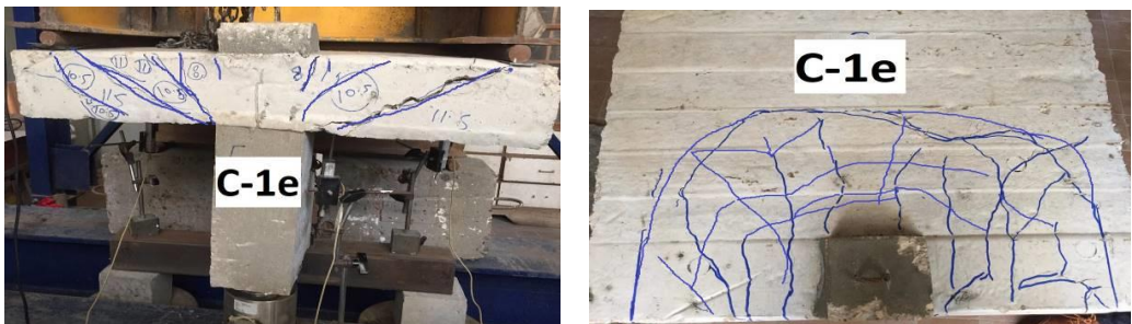
Fig.31. Pattern of cracking for specimen (C-1e).
