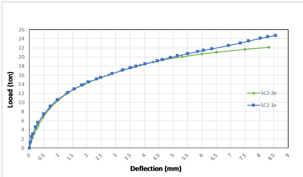
Fig. 21 Effect of load eccentricity value (e) variation with two rows of (CFRP) strengthening stirrups.
