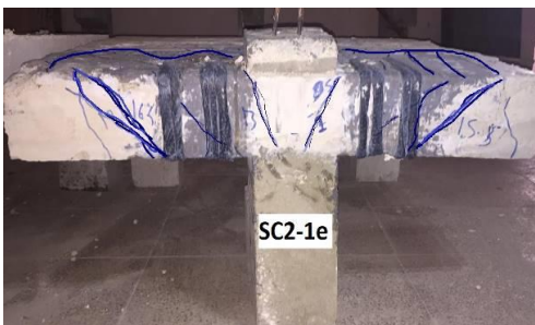
Fig. 35. Pattern of cracking for specimen (SC2-1e).
