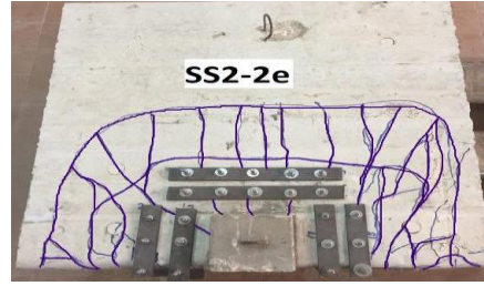
Fig. 44. Pattern of cracking for specimen (SS2-2e).
