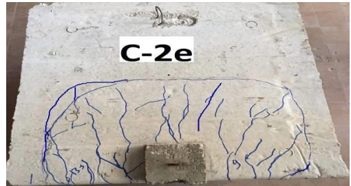
Fig. 32. Pattern of cracking for specimen (C-2e).
