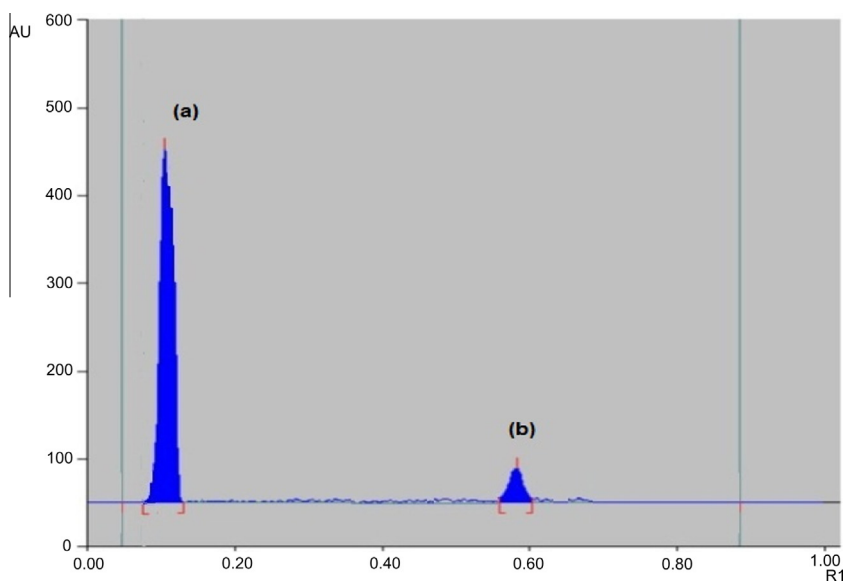
Figure 5 2D TLC chromatogram of (a) 4 µg/band of SCG and (b) 0.2 µg/band FLU using chloroform:methanol:toluene:triethylamine in ratio of (5:2:4:1 v/v/v/v) as developing system.
