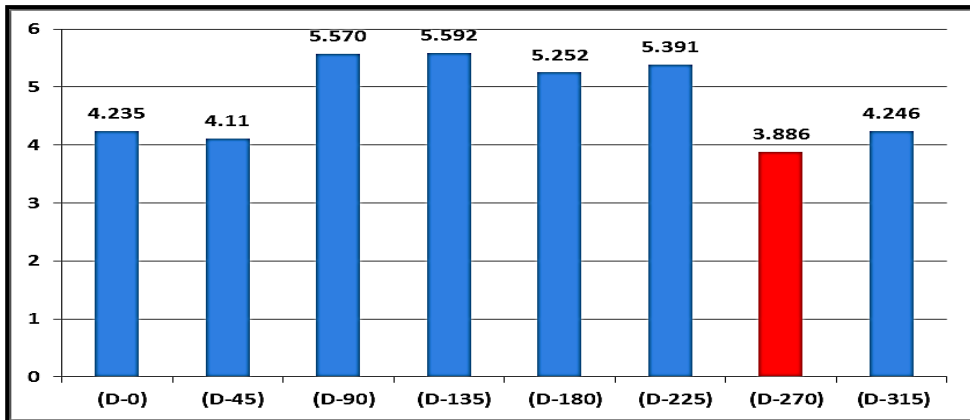
Fig.10 Average PMV at the two recording points in the outer urban space of the residential group (D) at 4:00 pm.
