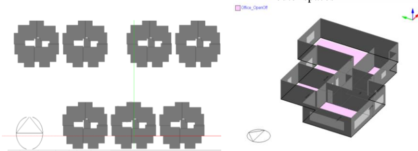
Fig27. shows the N-45 layout and 3D plan model (indoor) on the Design Builder Program
