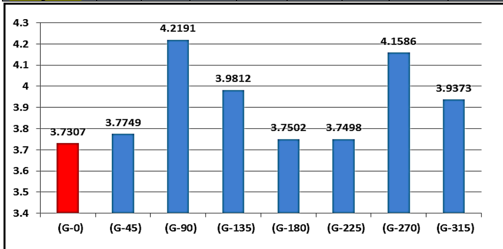
Fig.8 Average PMV at the two recording points in the outer urban space of the residential group (G) at 4:00 pm, source: Authors by Envi-met program
