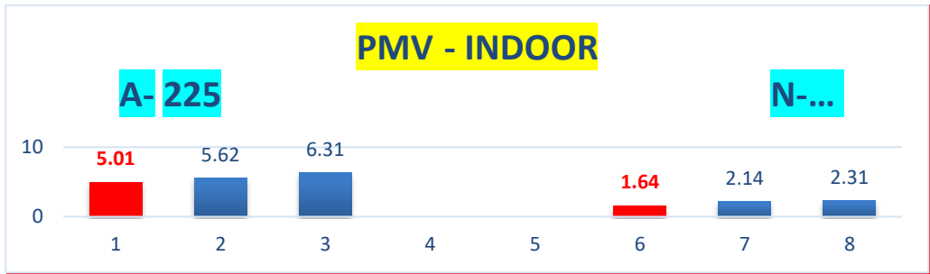
Fig. 32 shows a comparison chart between the three-point recording of thermal comfort PMV from within the spaces that overlook the outer space of the two models.
