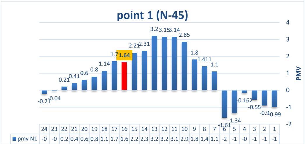
Fig.28 shows PMV measurement for point 1(N45-N1) at 4pm
