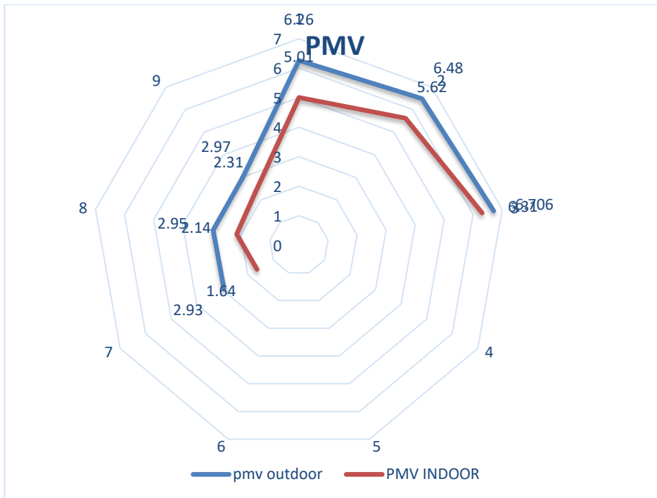
Fig. 34 shows a comparison curve between of thermal comfort PMV from indoor and outdoor the spaces of the two models.
