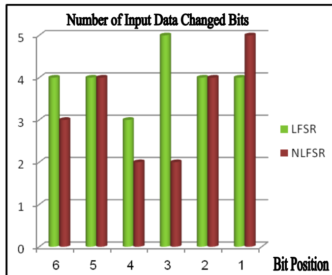
Fig. 7: Input Data Masking Effect Analysis
