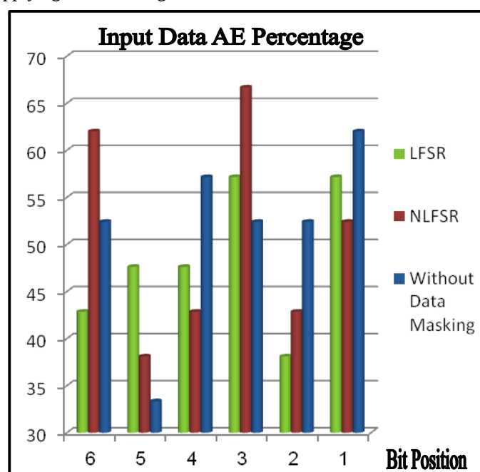
Fig. 8: Input Data Avalanche Effect Analysis
