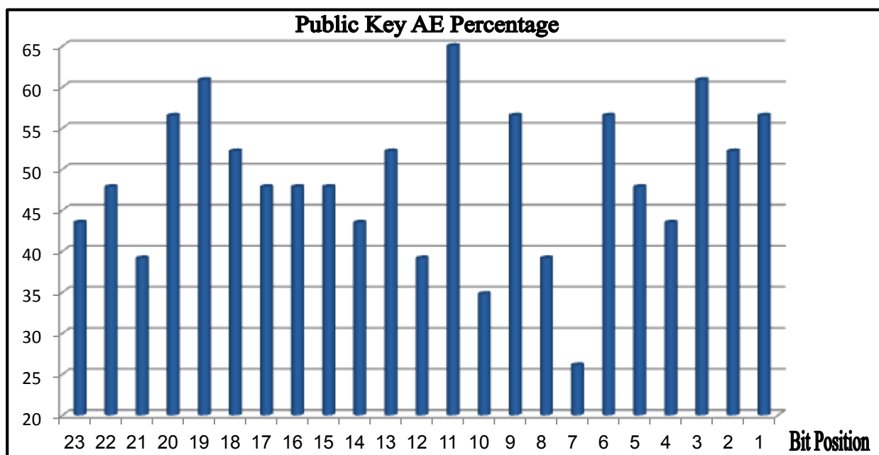
Fig. 9: Public Key Avalanche Effect Analysis
