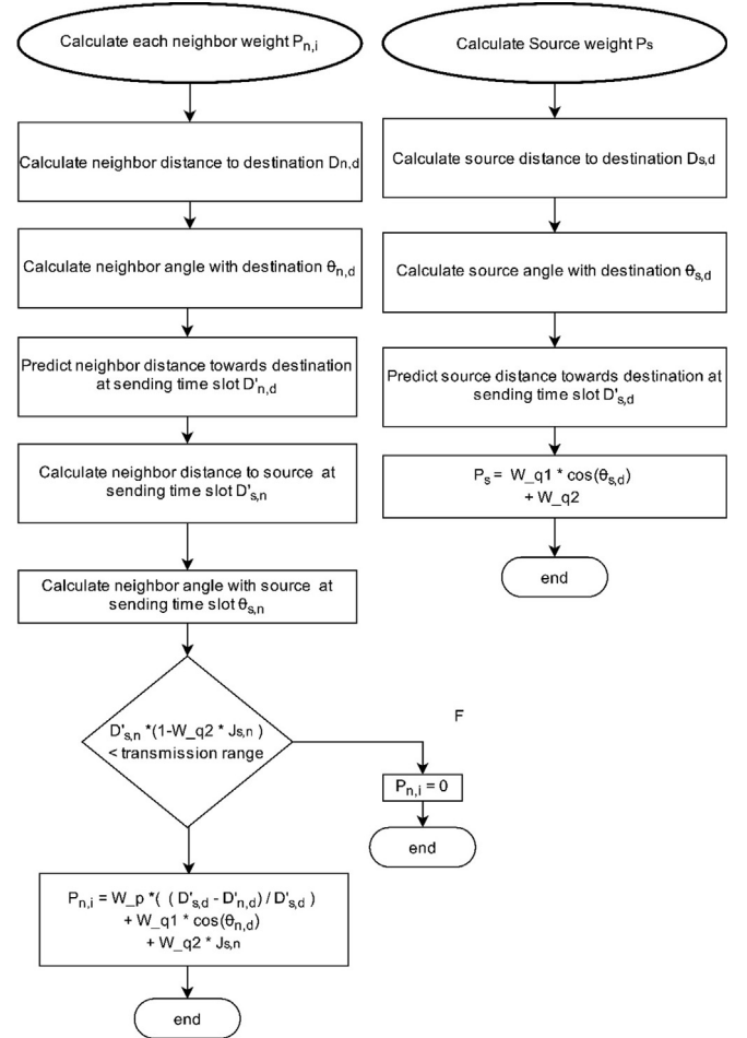
Fig. 6b. The OPBRP calculations steps flow chart.
