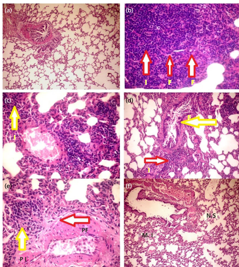
Figure 5 Histopathological examination of the inflammation of the right lung tissues stained with haematoxylin and eosin (H&E) (40 \times ). Control (a) without inflammation, ovalbumin-sensitized guinea pigs with bronchial asthma (b–d), and ROSI treated groups (e–f). The extent of inflammation indicated by I: inflammatory infiltration F: overt features of fibrosis with PI: partial peri-vascular fibrosis, NS: no signs of fibrosis, and MF: features of minimal monocytic inflammatory infiltrate.
