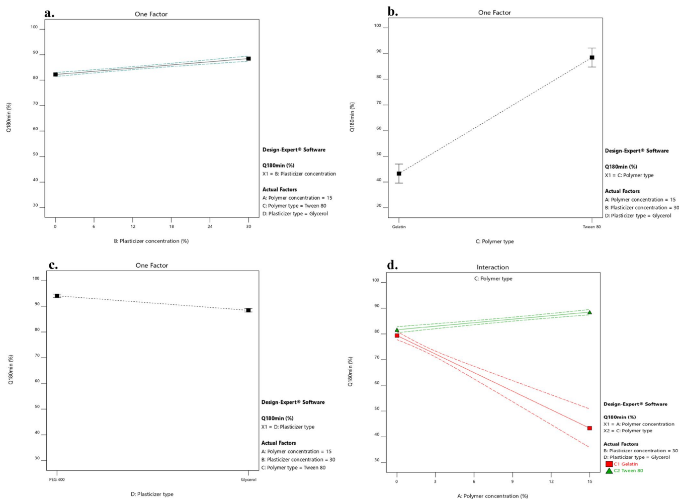
Figure 5. Impact of the independent variables and the interactions on the percentage of LN2 release after 180 minutes. a. X_2 : plasticizer concentration, b. X_3 : polymer type, c. X_4 : plasticizer type, and d. X_1/X_3 : polymer concentration/polymer type.
