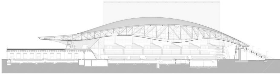
fig. 2 Section through the center, showing the structural details [31]
