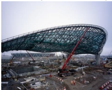
fig. 3 The structural steel frames and the transfer of the loads [32]
