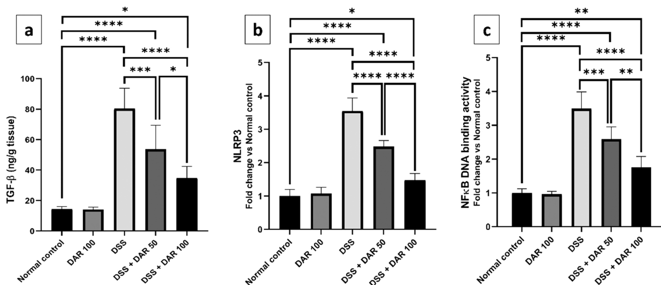
Fig. 3. Effect of DSS and/or diacetylrhein on the expression of inflammation-related factors in colon tissue: a) TGF- \beta , b) NLRP3 and c) NF- \kappa B DNA binding activity. * P < 0.05 , ** P < 0.01 , *** P < 0.001 , **** P < 0.0001 .
