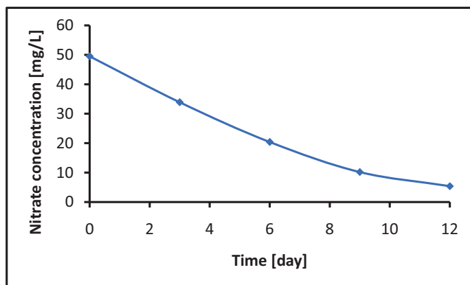
Fig. 41.3 Consumption of nitrate with time at 25 °C
