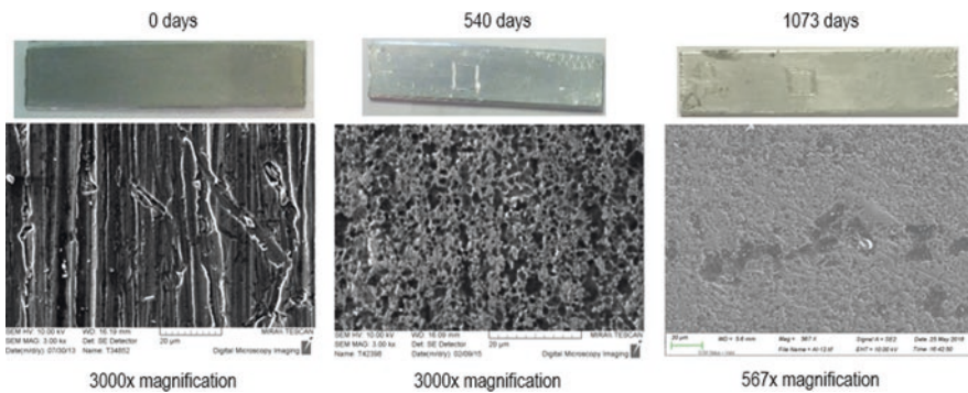
Fig. 57.5 Aluminium immersed in Micronal®
