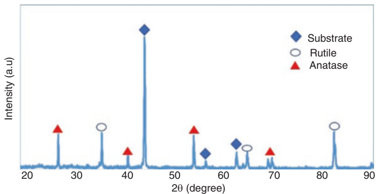
Fig. 79.9 XRD pattern of the \text{TiO}_2/\text{NaCl} porous film deposited sample (50 mm)
