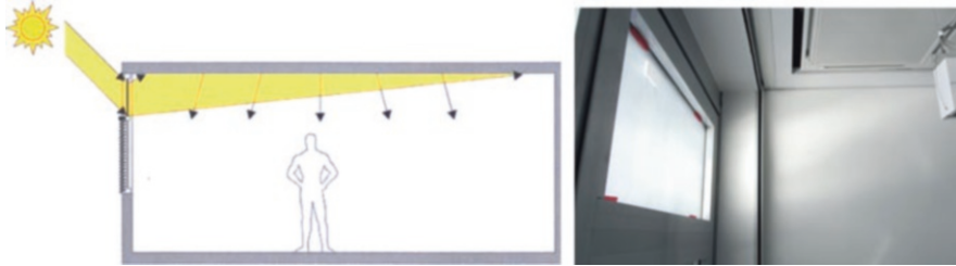
Fig. 50.1 Left: Principle of redirecting solar light from the upper window area to a reflecting ceiling and deep into the room. Solar protection in the lower window area, e.g., shading or glass coating. Right: Prototype in test room of Fraunhofer IBP, Stuttgart
