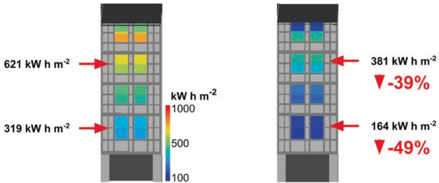
Fig. 56.6 Influence of reflection on the cumulative annual irradiance transmitted through the windows of one building on the north facade
