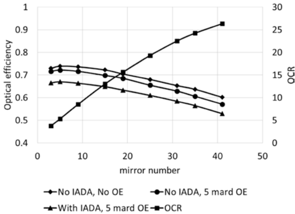
Fig. 26.5 Variation of optical efficiency and OCR against mirror number
