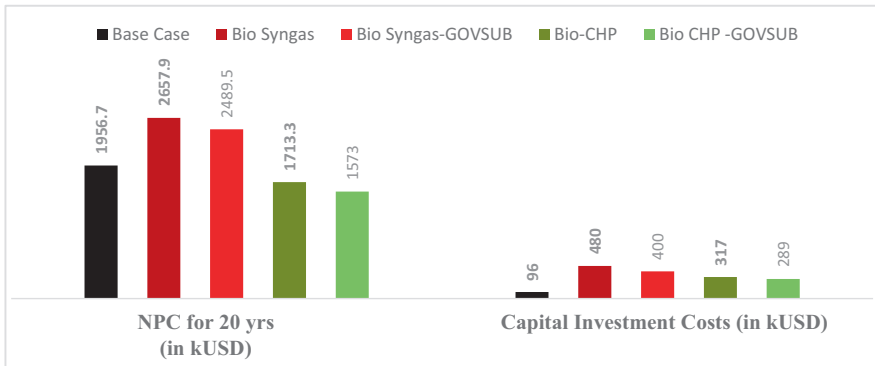
Fig. 74.3 NPC for 20 years and capital investment costs of all cases
