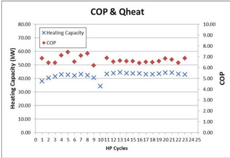
Fig. 60.3 R245fa performance for a high evaporator temperature heat pump providing heat to hydronic radiators at > 60 °C
