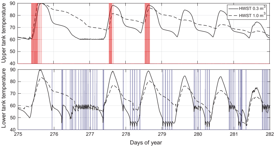
Fig. 40.7 Solar heat collector behaviour in two tanks with perfect forecasting (red highlight, electric heating element operation times for 1 m 3 tank; purple highlight, heat pump operation times for 0.3 m 3 tank)
