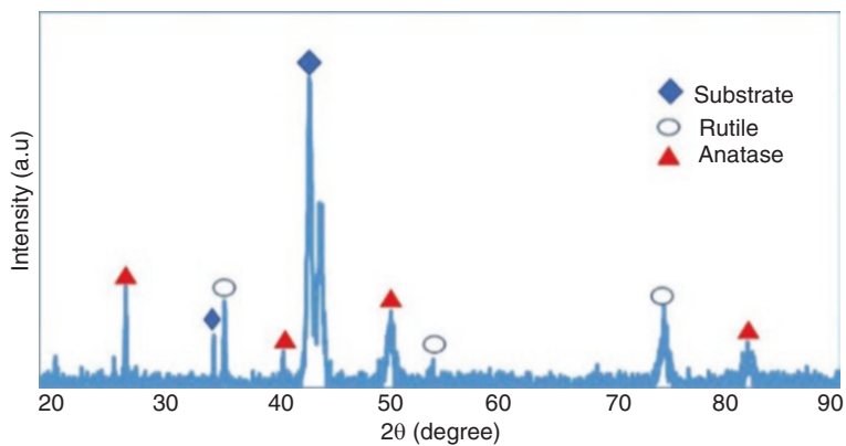
Fig. 79.11 XRD pattern of the \text{TiO}_2/\text{NaCl} porous film deposited sample (70 mm)
