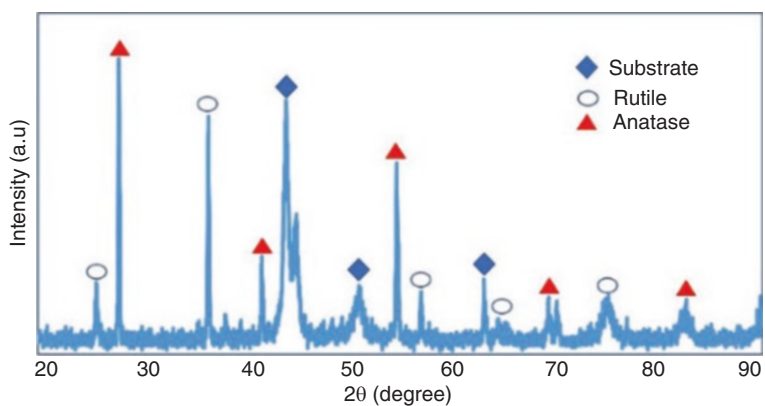
Fig. 79.10 XRD pattern of the \text{TiO}_2/\text{NaCl} porous film deposited sample (60 mm)
