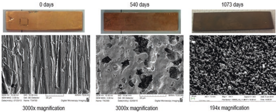
Fig. 57.3 Copper immersed in Micronal®
