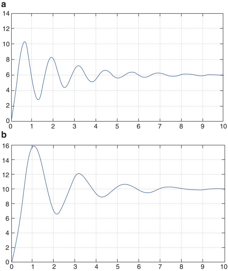
Fig. 38.8 (a) Output voltage of the DC–DC boost converter for V_{pv} = 3 V and \alpha = 0.5 . (b) Output voltage of the DC–DC boost converter for V_{pv} = 3 V and \alpha = 0.7
