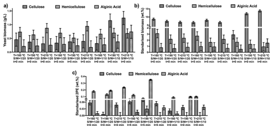
Fig. 76.3 Fermentation results: total yeast biomass concentration (a), total yeast biomass as a function of the amount of solubilised material (b) and 2PE production as a function of solubilised material (c) for the hydrolysates produced from cellulose, hemicellulose and alginic acid. Bars are Fisher's least significant difference (LSD) intervals with 95% confidence
