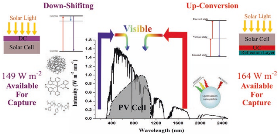
Fig. 58.1 Schematic overview of the spectral conversion approach for photovoltaic technologies. Indicating the solar irradiance available for capture (black line) as well as the two main types of spectral converters available (downshifting—violet, and up converters—red) and their corresponding electronic band structure. The total amount of irradiance available for capture and conversion with each type of converter is also presented. Please note the \text{Wm}^{-2} values presented are reflective of the those available for mc-Si technology, and are not reflective of the energy available for capture by alternative PV technologies, whose spectral responsivity profile will be different
